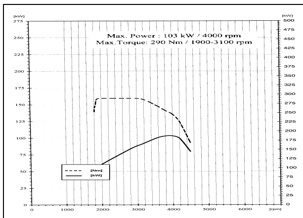
Manufacturer's values: Volvo: upper curve = torque, right-hand scale, [Nm]; lower curve = motor power, left-hand scale, [kW].
