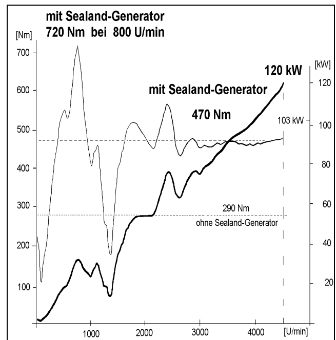
Measurements with the Sealand Generator: thin curve = torque, left-hand scale, [Nm]; bold curve = motor power, right-hand scale, [kW].
